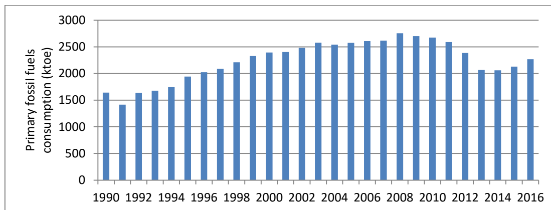
Figure 2.6. Primary consumption of fossil fuels in ktoe, 1990-2016
