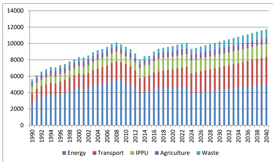
Figure 5.3. Total BaU GHG emissions by sector (Gg CO2 eq.) 1990-2040
