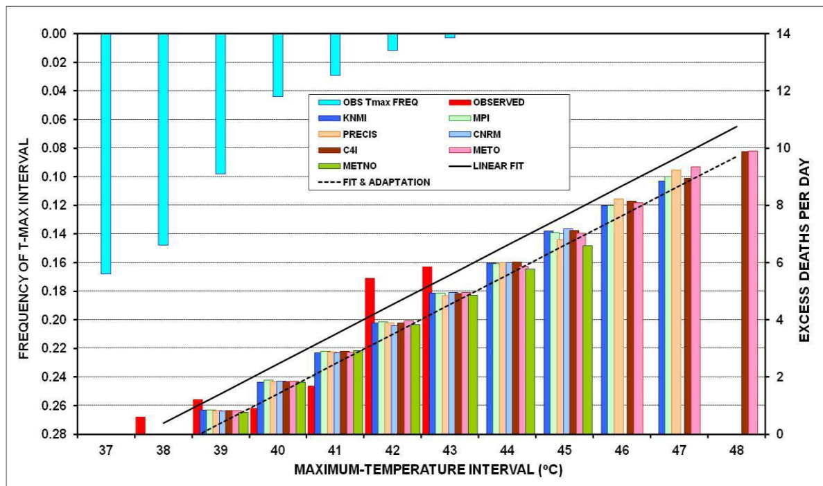
Figure 6.21. Excess deaths (right axis; model and observation bars for present and future climate with adaptation) and daily temperature frequencies (left axis; light blue bars) in Cyprus for the future period 2021-2050
