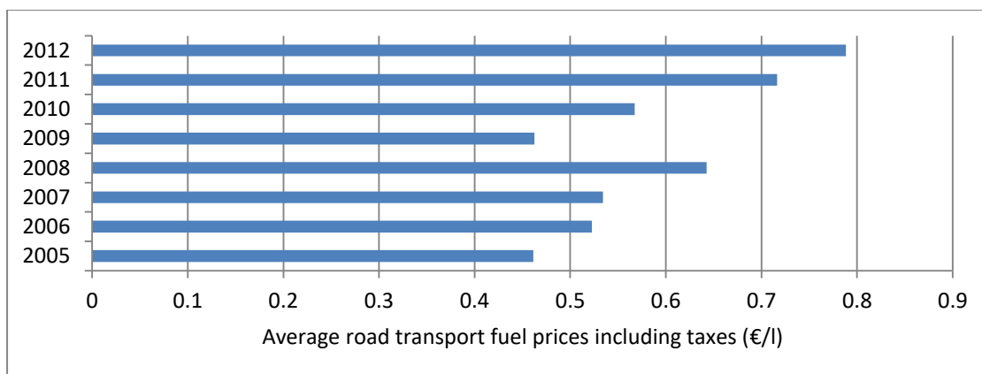
Figure 2.12. Average road transport fuel prices including taxes in €/litre, 2005-2012
