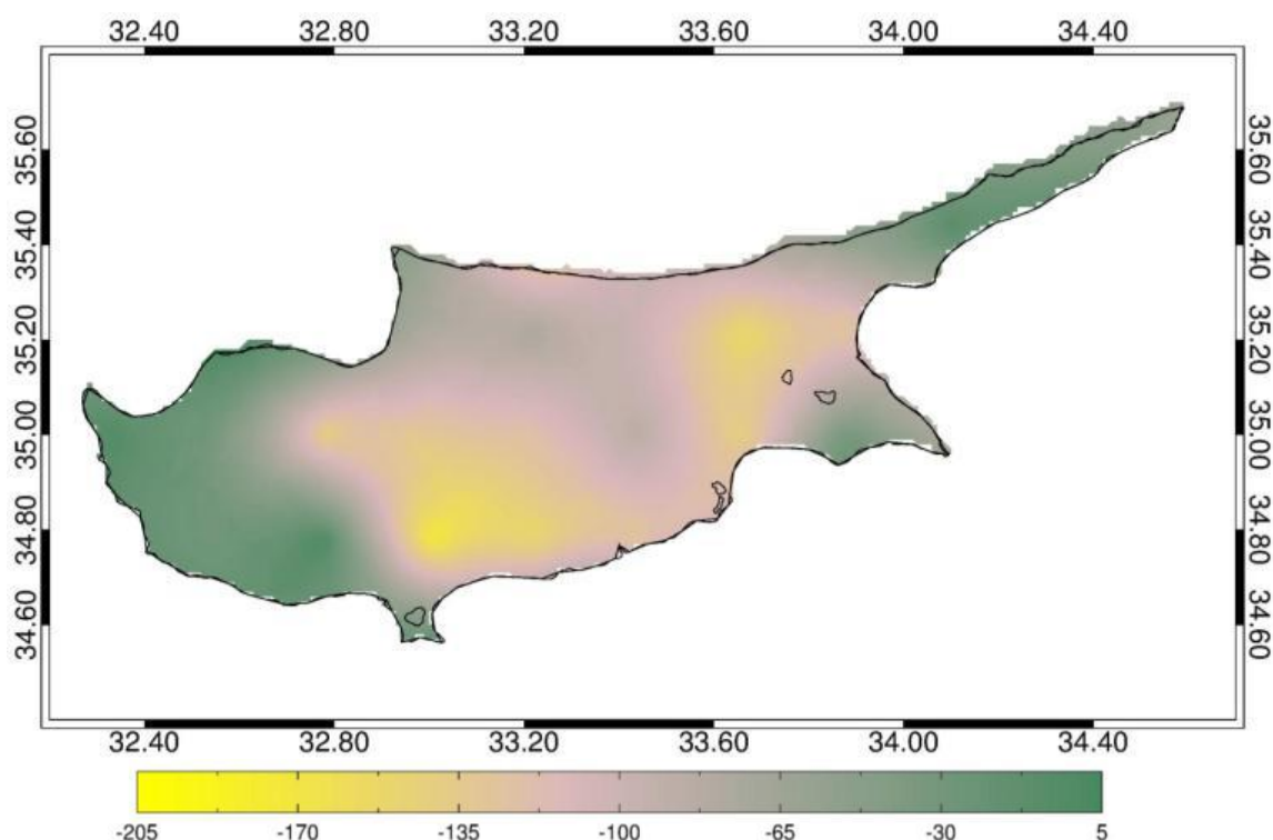
Figure 6.38. Changes in maximum length of dry spell ( RR < 0.5\text{mm} ) between the future (2021-2050) and the control period (1961-1990)
