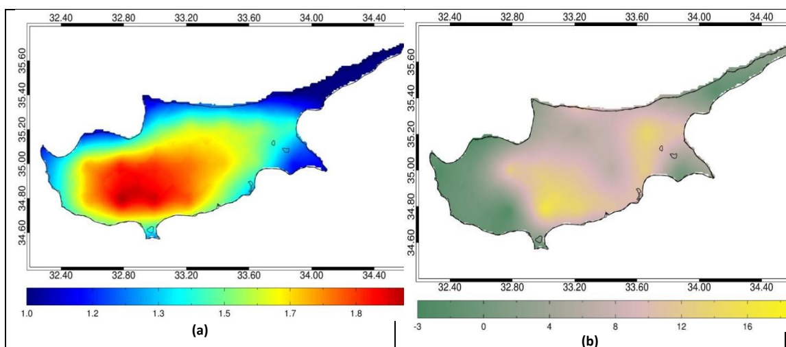
Figure 6.29. Changes in (a) average annual maximum temperature and (b) maximum length of dry spell ( RR < 0.5\text{mm} ) between the future (2021-2050) and the control period (1961-1990)
