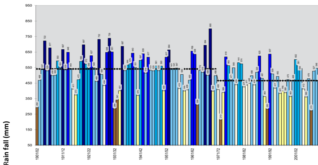
Hydrological years 1901/02 -2010/11
