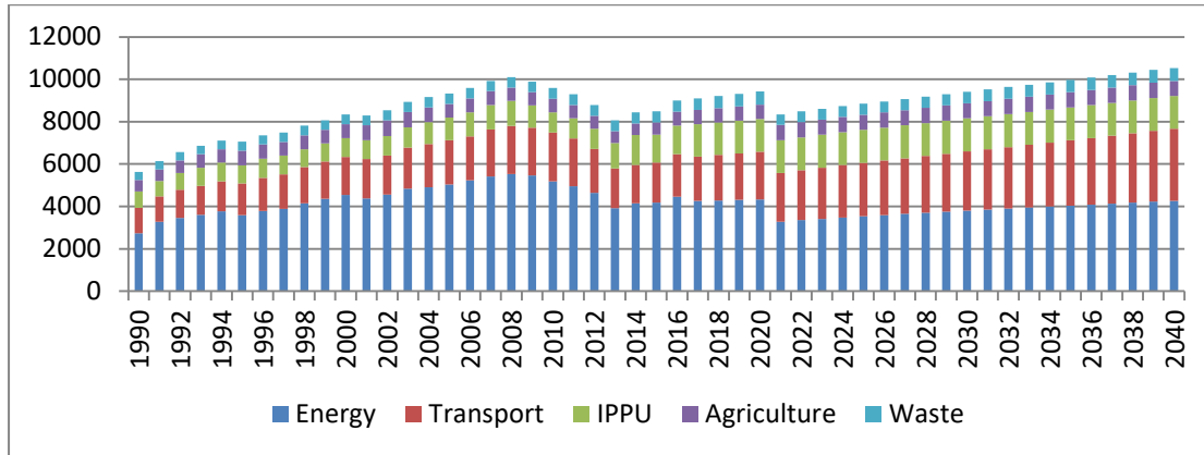
Figure 5.5. Total WEM GHG emissions by sector (Gg CO2 eq.) 1990-2040
