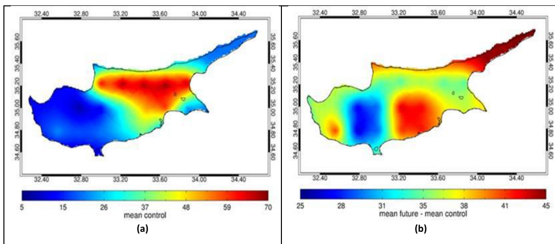
Figure 6.22. Maximum length of Humidex > 38°C (a) for the control period (1960-1990) and (b) the near future (Future – Control period), PRECIS RCM model
