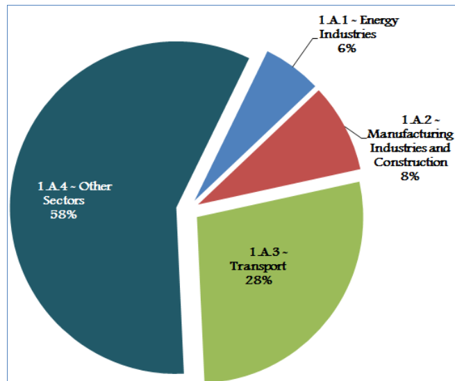
Figure 4-9 shows percentage contribution of emissions by source categories in the energy sector.
