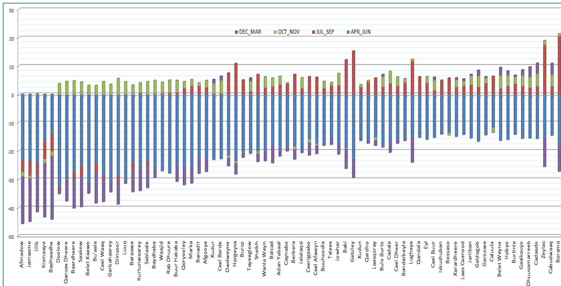
Figure 6-32 Seasonal Variability (mm/decade) of Rainfall in Various Districts
