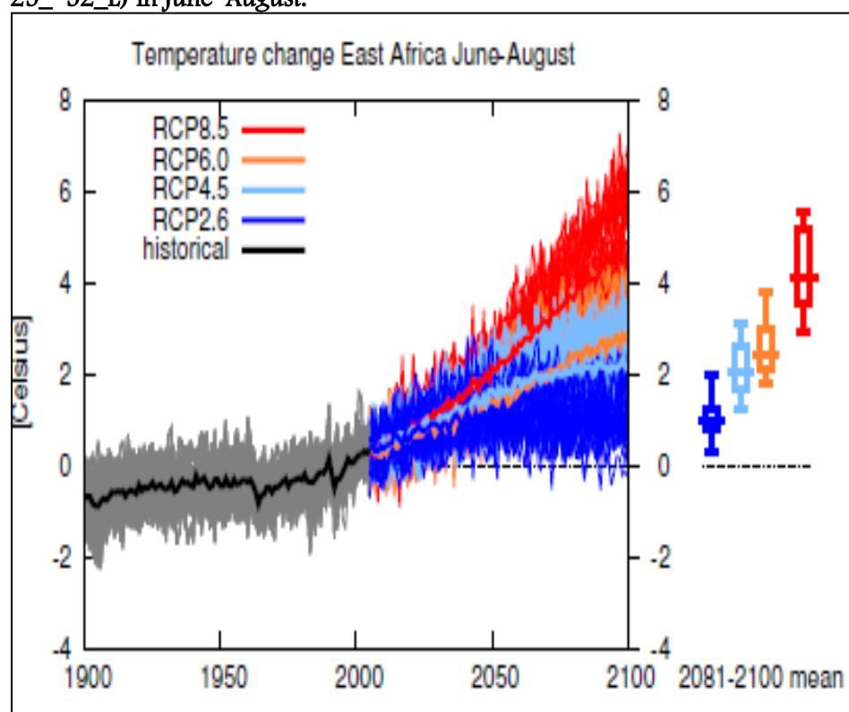
Figure 6-7 Time Series of Temperature Averaged over Land Grid Points in East Africa (11.3_S–15_N, 25_–52_E) in June–August.
