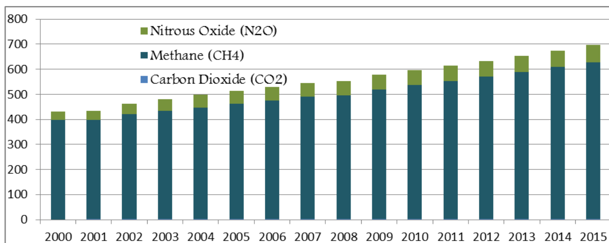
Figure 4-25 the trends of emissions (in Gg) by gas
