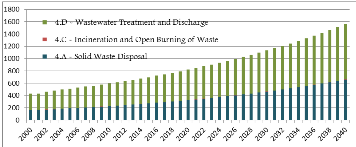
Figure 4-28 Projected (BAU) Emissions (in Gg) for the Wastes Sector
