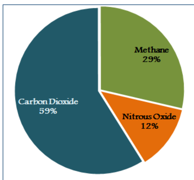
Figure ES 1-2 Year 2015 Emissions Percentage by Sector and Gas
