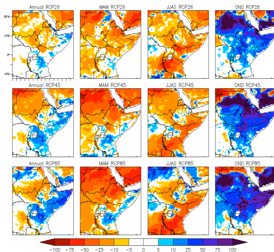
Figure 6-14 Projected rainfall changes over GHA by 2070s
