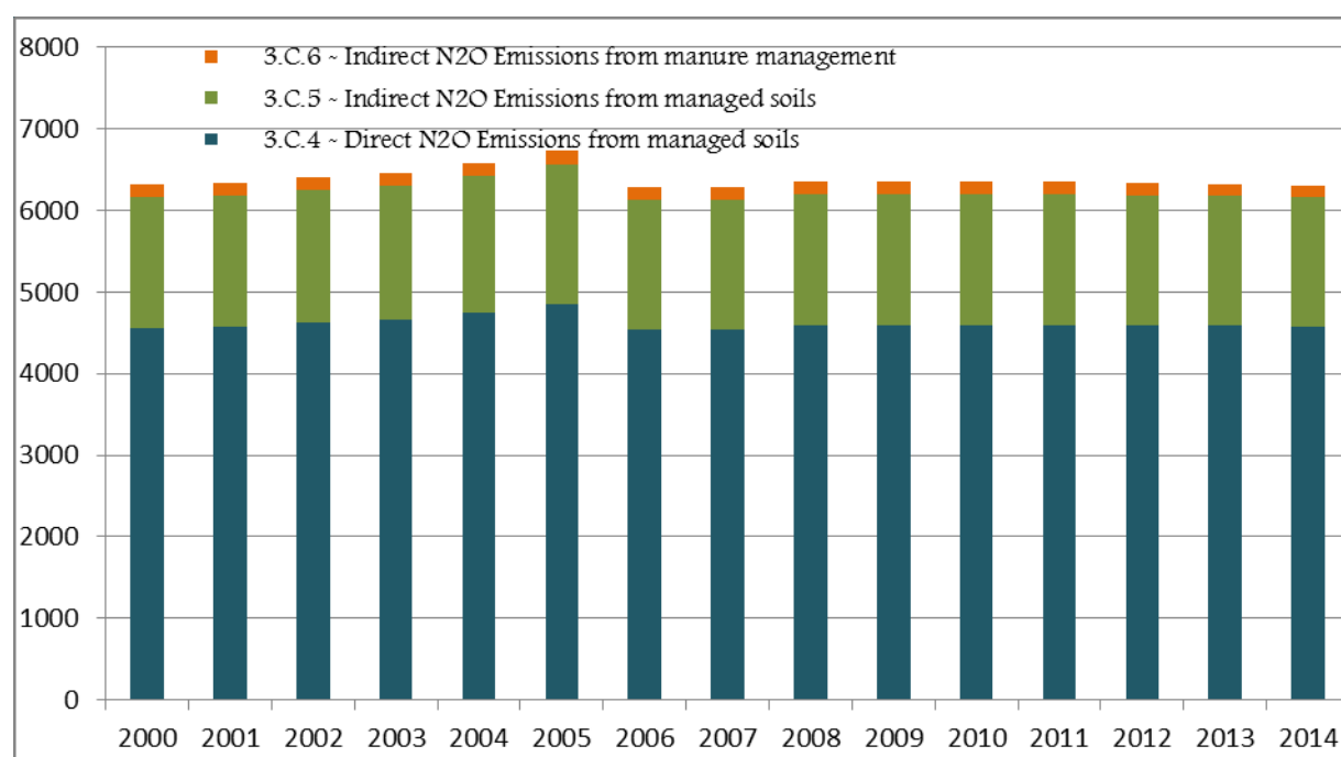
Figure 4-20: The trend Nitrous oxide emissions (in Gg) by source category
