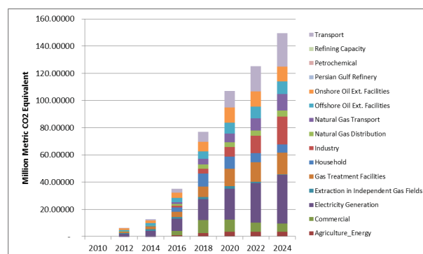
Figure (3.6): Contribution of Energy Subsectors in Total Greenhouse Effect Reduction (BAU vs. MIT)
