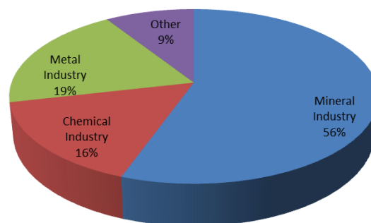
Figure (2.5): Contribution of Different Sources to CO 2 Emissions from IPPU
