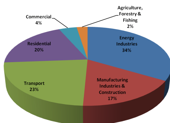
Figure (2.3): Contribution of Different Energy Sub-sectors to CO 2 Emissions in 2010
