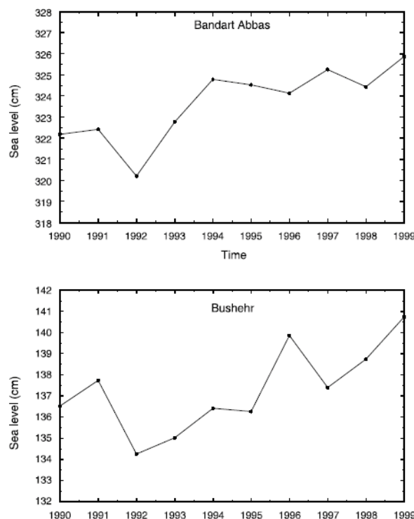
Figure (4.23): Sea Level Changes in Bandar Abbas and Bushehr during 1990 to 1999 (Hossenibalam et al., 2007)
