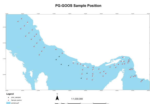
Figure (5.7): The Position of Stations in PG-GOOS Research Cruise (2012-2014)
