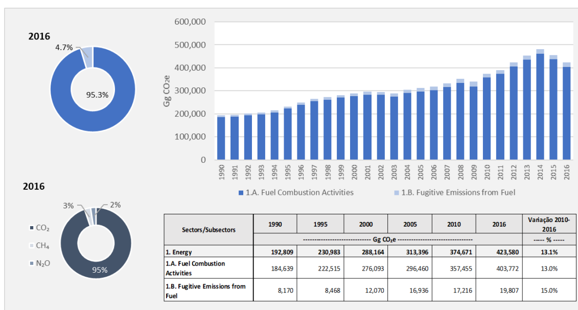
Figure 2.14. Emissions of the Energy sector, in CO 2 e, by subsector from 1990 to 2016
