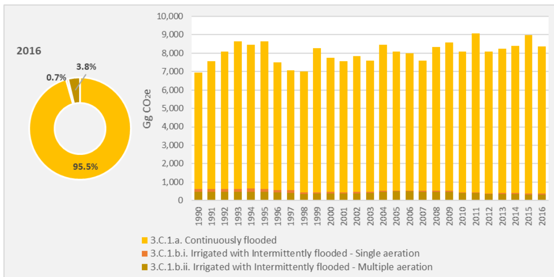
Figure 2.29. CH 4 emissions from rice cultivation (3.C), with the main types of irrigation, from 1990 to 2016
