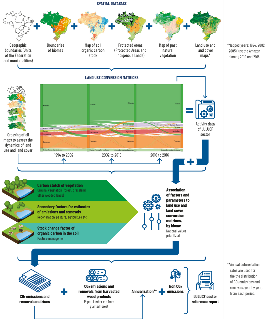
Figure 2.35. Flowchart of the methodology used to prepare the National Inventory of the LULUCF sector
