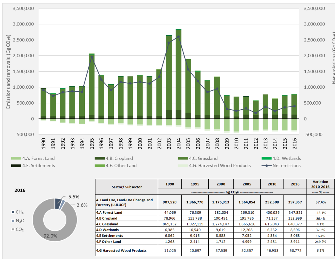
Figure 2.34. LULUCF sector emissions, in CO 2 e, by subsector, from 1990 to 2016
