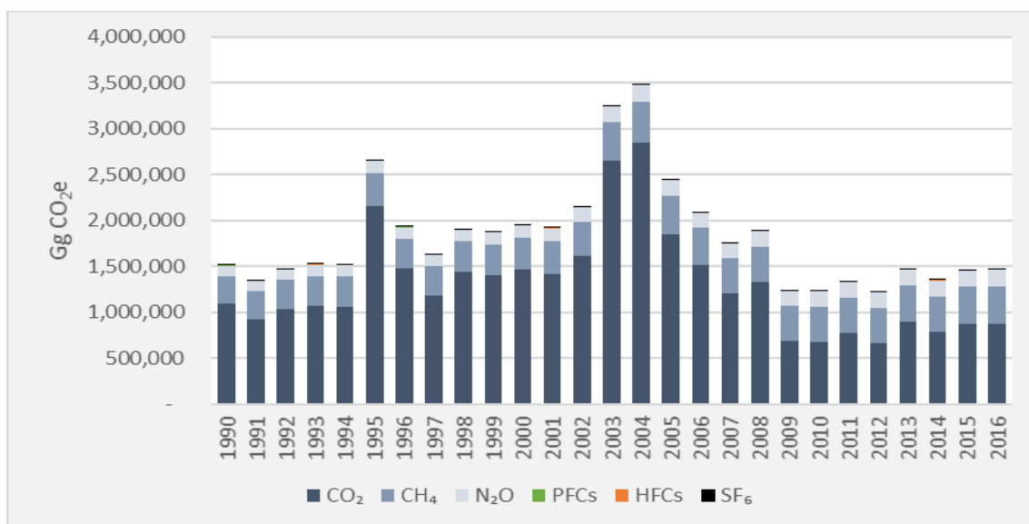
Figure 2.5. Result of the evolution of GHG emissions in Gg CO 2 e from 1990 to 2016.
