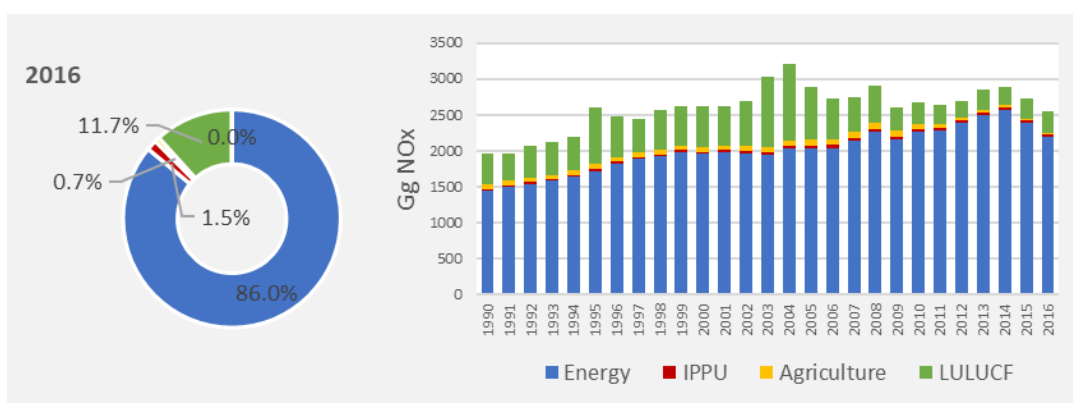
Figure 2.12. NO x emissions, from 1990 to 2016
