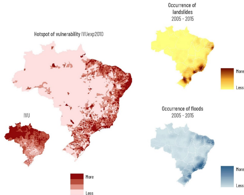
Figure 3.46. Hotspots for urban vulnerability and disasters. Own elaboration based on Cenad (2018) data and IBGE (2010).
