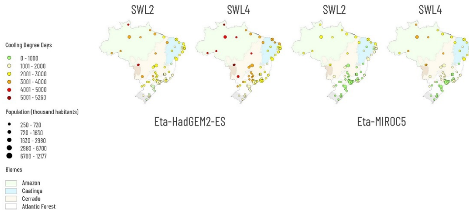
Figure 3.28. GDRs' results for Eta-HadGEM2-ES and Eta-MIROC5 models for SWL2 and SWL4.
