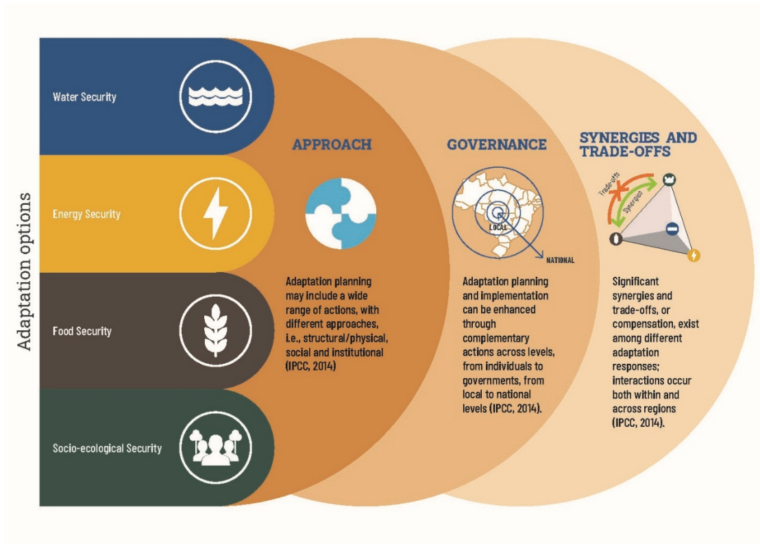
Figure 3.59. Integrated adaptation planning.
