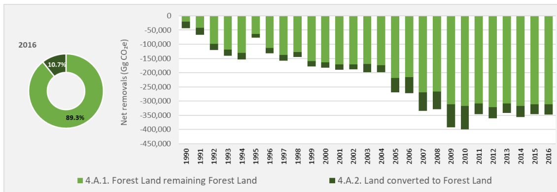
Figure 2.36. Net removals of the categories of the Forest Land subsector (4.A), in CO 2 e, from 1990 to 2016.
