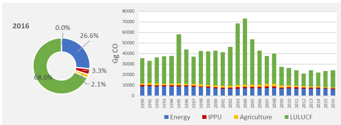
Figure 2.11. CO Emissions, from 1990 to 2016
