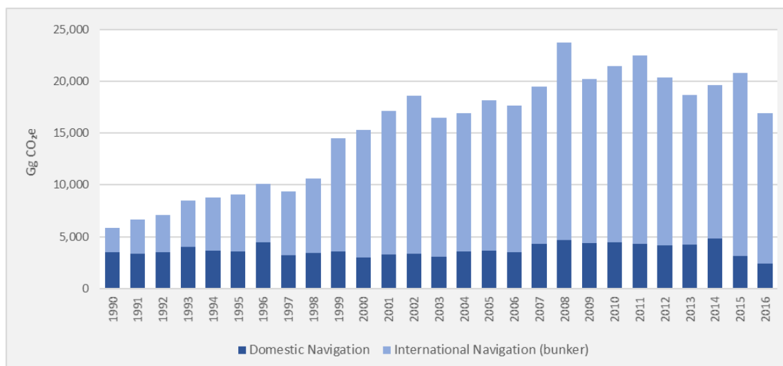
Figure 2.16. Historical series of CO 2 e emissions for domestic navigation and bunker, from 1990 to 2016
