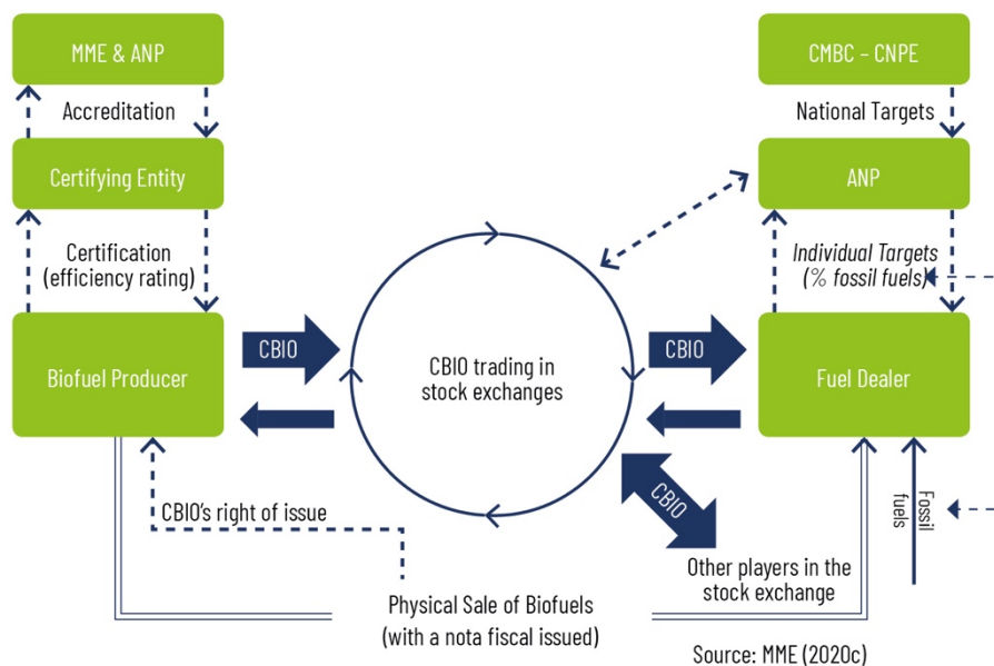
Figure 4.2. Operational flow for RenovaBio
