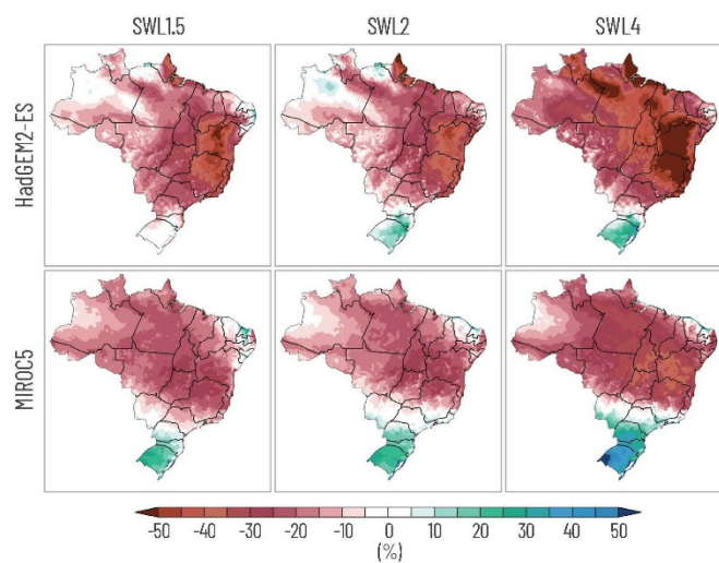
Figure 3.44. Precipitation projections: annual precipitation variation (%) compared to the reference period (1961-1990) according to the SWL1.5, the SWL2 and the SWL4 from each experiment carried out with the Eta model.
