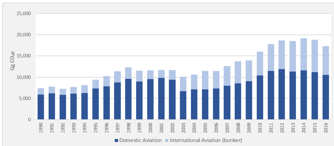
Figure 2.15. Historical series of CO 2 e emissions for domestic aviation and bunker, from 1990 to 2016
