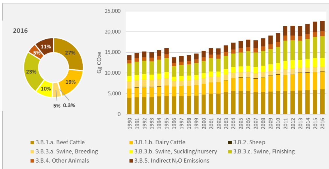
Figure 2.28. Emissions from Manure Management (3.B), in CO 2 e, of the main animal categories from 1990 to 2016
