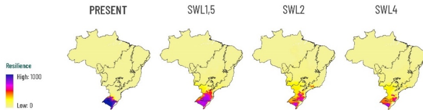
Figure 3.43. Projections of the Pampa Biome's resilience in the present and the scenarios SWL1.5, SWL2, and SWL4.
