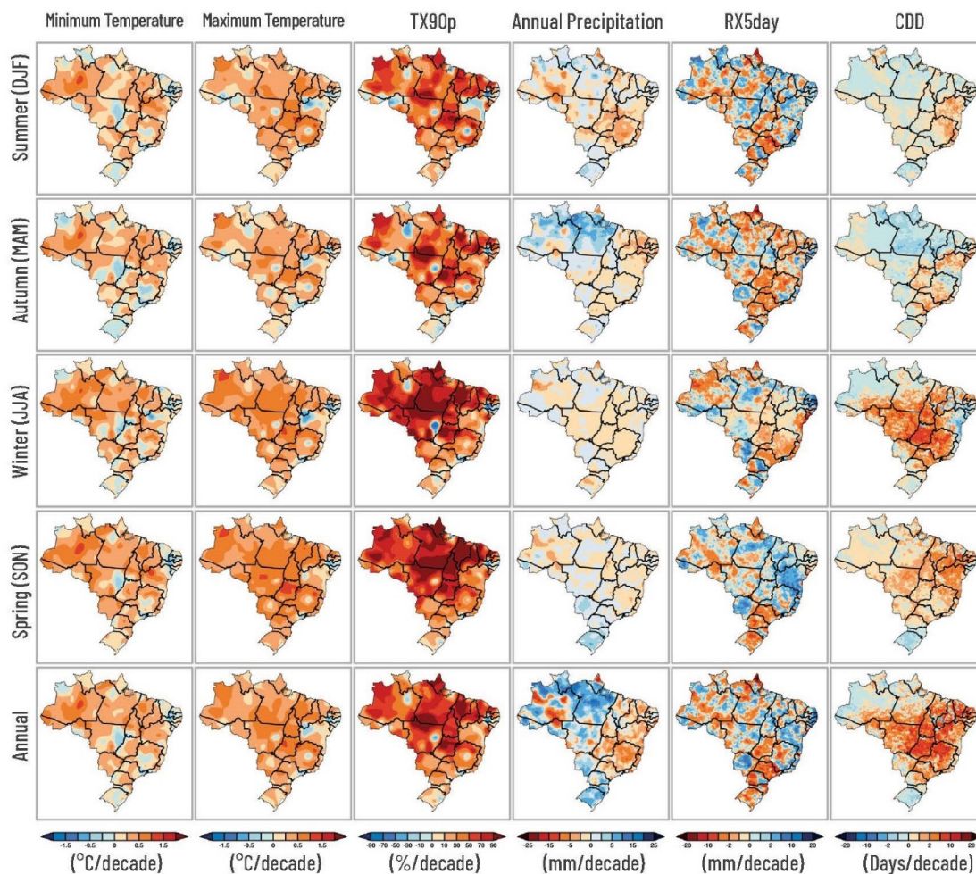
Figure 3.2. Trends noticed from the minimum and maximum temperatures (Celsius/decade); from the annual precipitation (mm/decade); from the number of days with maximum temperature over the percentile 90 – TX90p (%/decade); and maximum rainfall accumulated, between 1980-2018.
