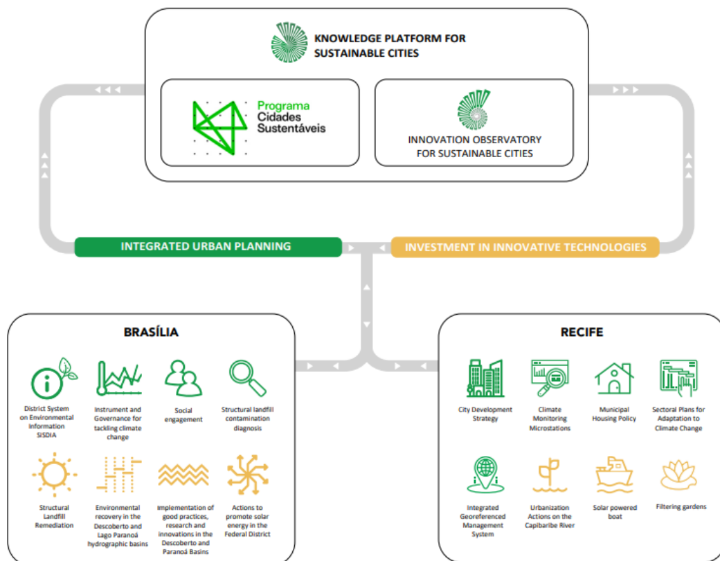
Figure 4.4. Action fronts of the CITinova Project
