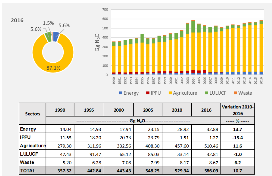
Figure 2.9. National N 2 O emissions, of all sectors, from 1990 to 2016.
