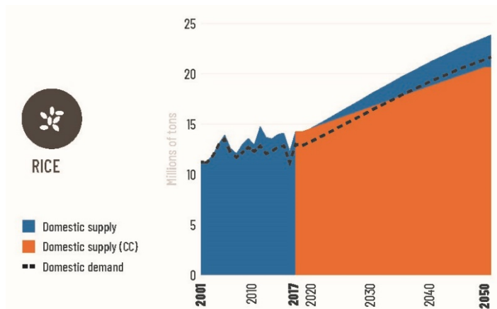
Figure 3.29. Projections of rice domestic supply “without” and “with” climate change (MC) (until 2050).
