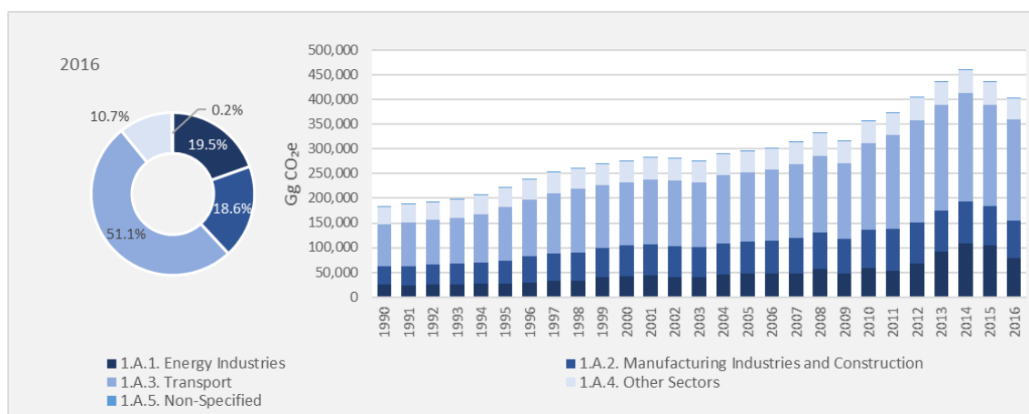
Figure 2.17. Emissions from Fuel Combustion Activities (1.A), in CO 2 e, by category from 1990 to 2016
