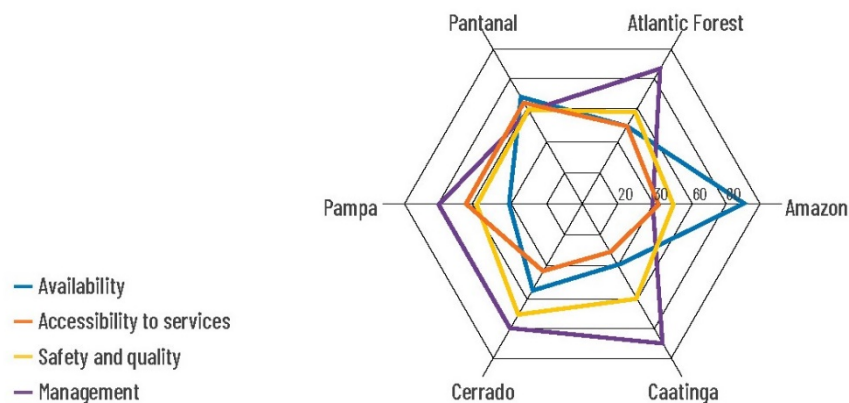
Figure 3.19. Median of each ISHmc dimension for each biome, the availability is simulated by Eta-HADGEM 2-ES model (Eta-MIROC5 model has shown a similar result) for the present climate (1961-1990).
