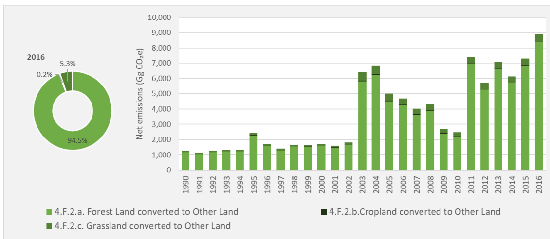
Figure 2.41. Net emissions of the subcategories of the Land converted to Other Land category (4.F.2) of the Other Land subsector (4.F), in CO 2 e, from 1990 to 2016
