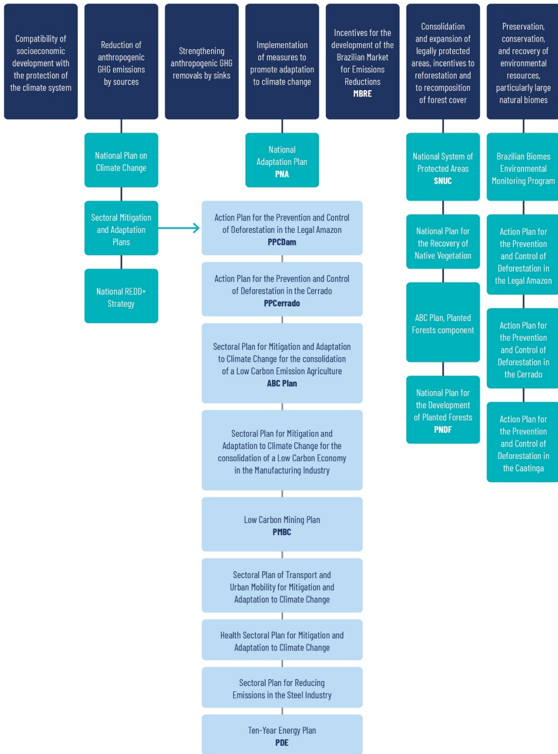
Figure 1.10. Institutional arrangement of the National Policy on Climate Change (PNMC).
