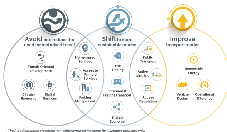
Figure 2: Avoid-Shift-Improve framework
