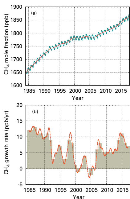
Figure 5. Globally averaged \text{CH}_4 mole fraction (a) and its growth rate (b) from 1984 to 2017. Increases in successive annual means are shown as the shaded columns in (b). The red line in (a) is the monthly mean with the seasonal variation removed; the blue dots and line depict the monthly averages. Observations from 126 stations have been used for this analysis.
