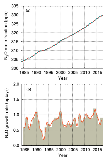
Figure 6. Globally averaged \text{N}_2\text{O} mole fraction (a) and its growth rate (b) from 1984 to 2017. Increases in successive annual means are shown as the shaded columns in (b). The red line in (a) is the monthly mean with the seasonal variation removed; in this plot it is overlapping with the blue dots and line that depict the monthly averages. Observations from 96 stations have been used for this analysis.
