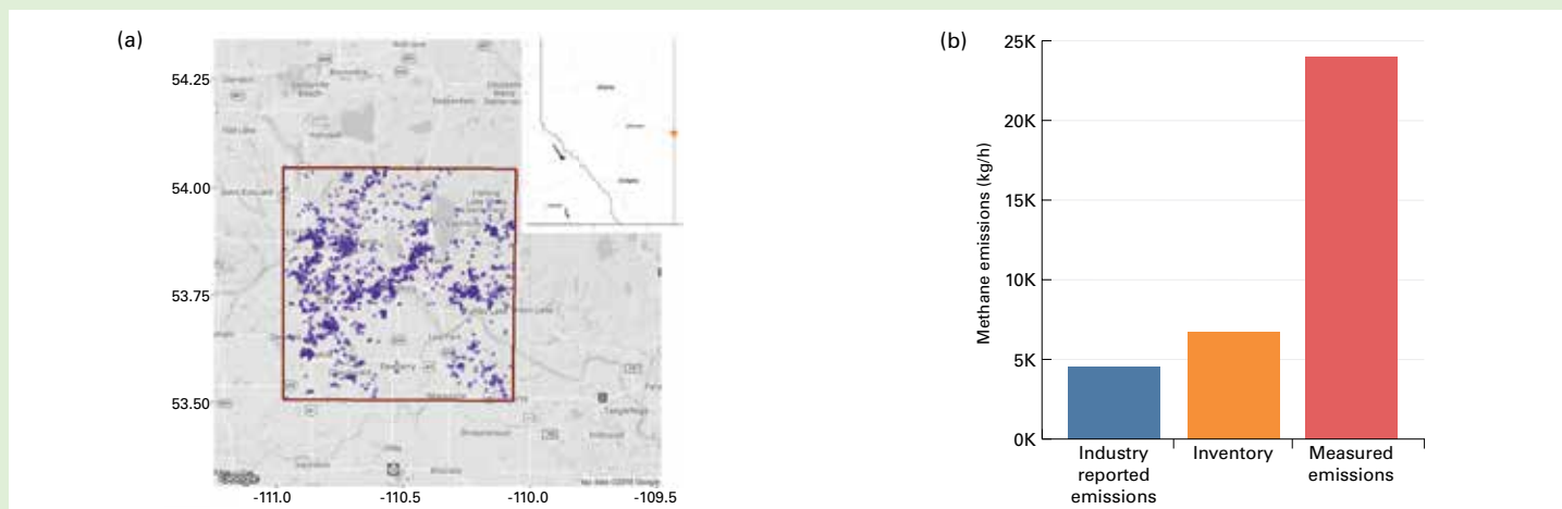
Figure 11. (a) Sampling region near Lloydminster, Alberta. The red box illustrates the source envelope where the aircraft took measurements. Purple dots inside the box represent active oil wells. (b) Comparison between measured \text{CH}_4 emissions and “bottom-up” estimates based on inventory and industry reports.
