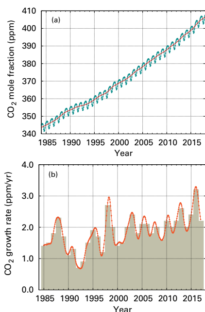
Figure 4. Globally averaged \text{CO}_2 mole fraction (a) and its growth rate (b) from 1984 to 2017. Increases in successive annual means are shown as the shaded columns in (b). The red line in (a) is the monthly mean with the seasonal variation removed; the blue dots and line depict the monthly averages. Observations from 129 stations have been used for this analysis.
