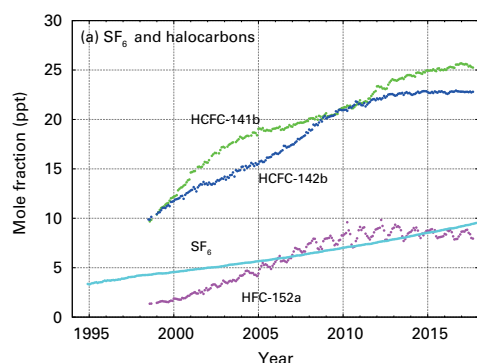
Figure 7. Monthly mean mole fractions of \text{SF}_6 and the most important halocarbons: (a) \text{SF}_6 and lower mole fractions of halocarbons and (b) higher halocarbon mole fractions. The numbers of stations used for the analyses are as follows: \text{SF}_6 (85), CFC-11 (23), CFC-12 (25), CFC-113 (21), \text{CCl}_4 (21), \text{CH}_3\text{CCl}_3 (24), HCFC-141b (9), HCFC-142b (14), HCFC-22 (13), HFC-134a (10), HFC-152a (9).
